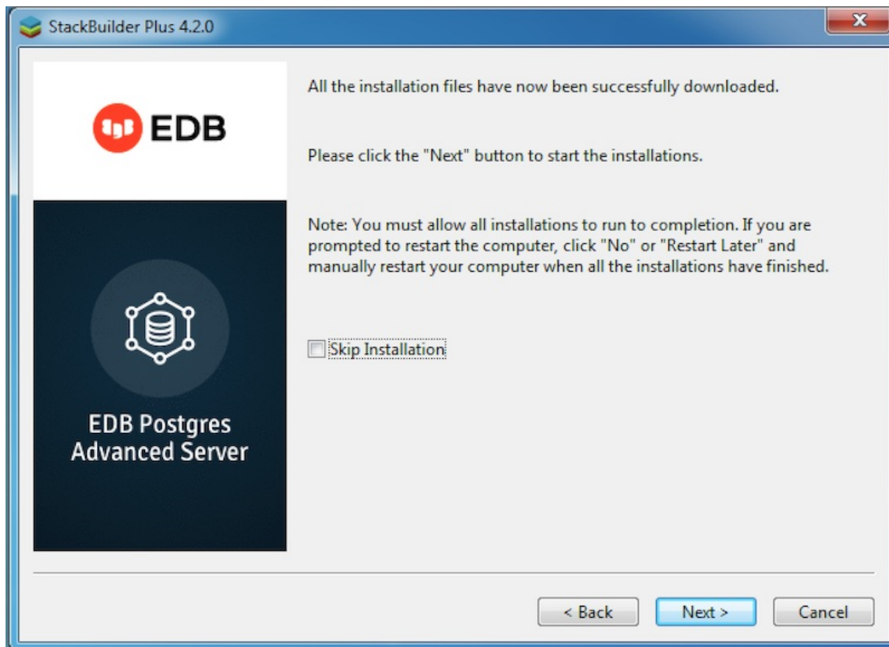
Fig. 2: Installing Slony
