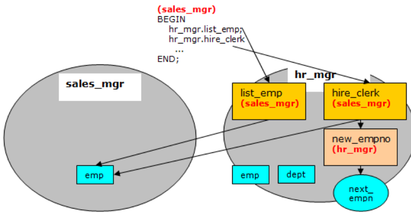
Fig. 1: Invokers Rights Programs
