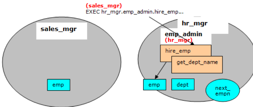
Fig. 3: Definer's Rights Package
